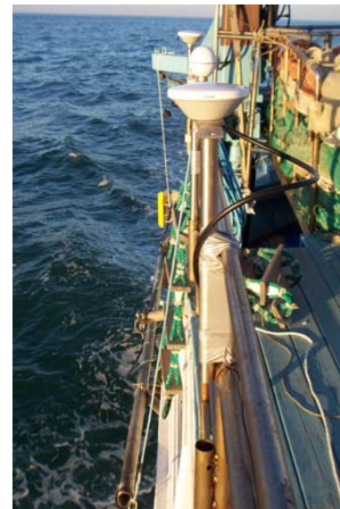
Survey boat and detail of sidemount arrangement
